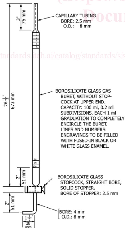
FIG. 3 Gas Buret
