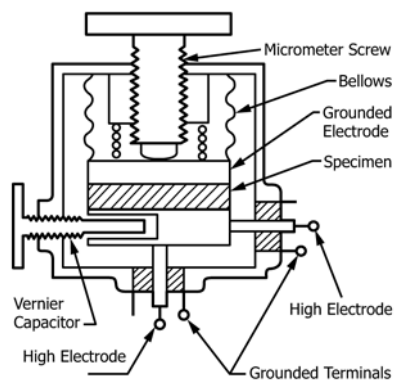
FIG. 9 Micrometer-Electrode System
