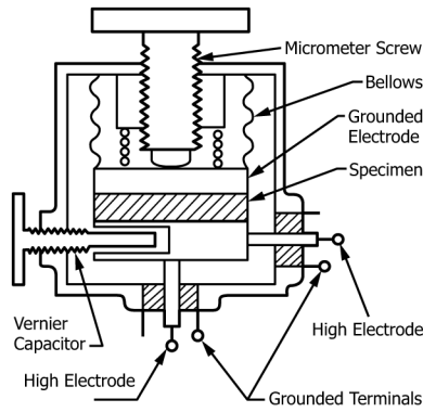
FIG. 109 Micrometer-Electroder System
