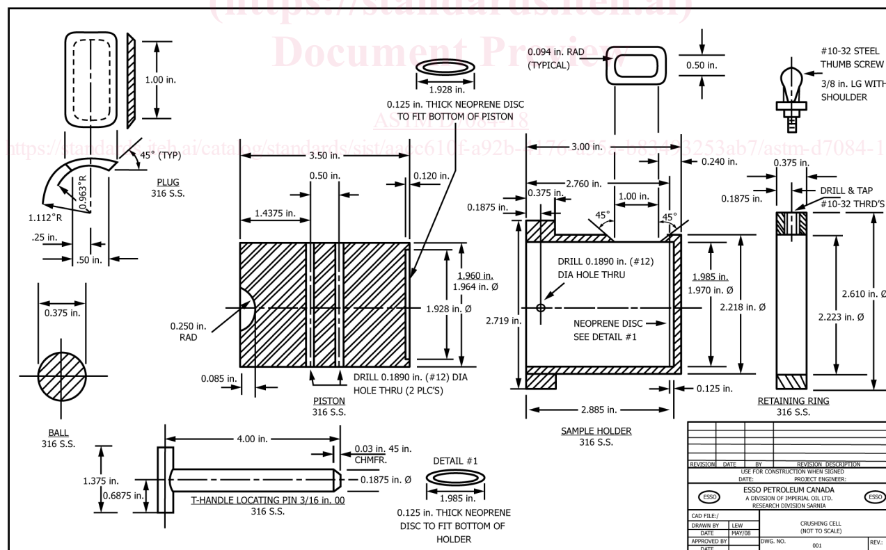
FIG. 1 Test Cell
