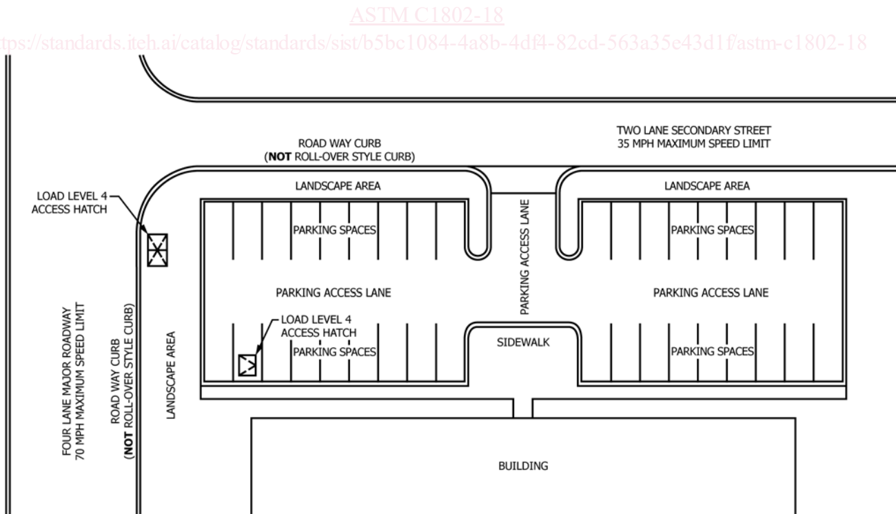
FIG. 4 Plan Showing Appropriate Locations for Load Level 4 Access Hatches—Occasional Truck Traffic
