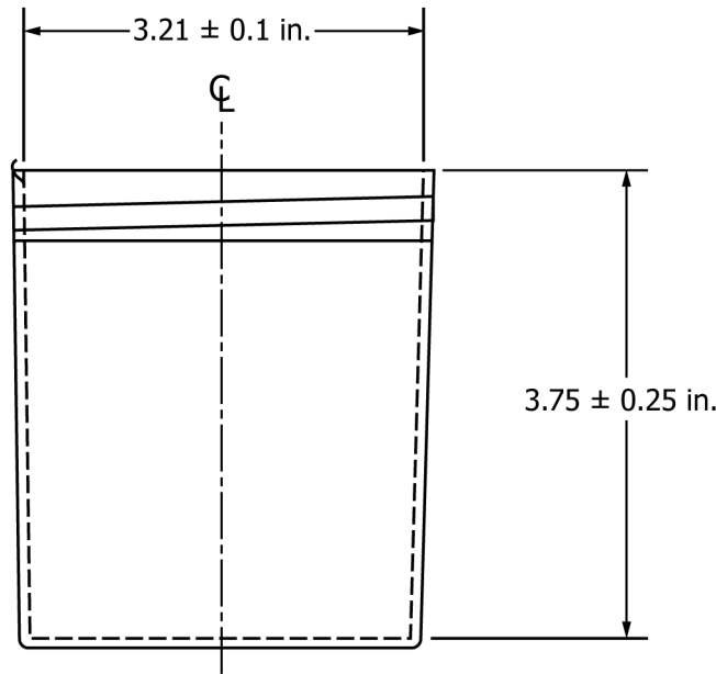
Test Jar Specifications Inner Diameter Range: 3.11–3.31 in. (79–84 mm) Inner Diameter Range: 3.11 in. – 3.31 in. (79 mm – 84 mm) Inner Height Range: 3.5–4.0 in. (89–102 mm) Inner Height Range: 3.5 in. – 4.0 in. (89 mm – 102 mm)
