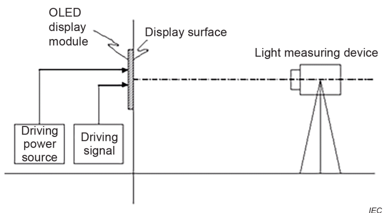
Figure 1 – Measuring system and arrangement
