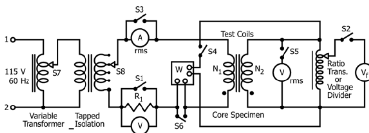
FIG. 1 Basic Circuit for the Measurement of Core Loss and Exciting Volt Amperes
