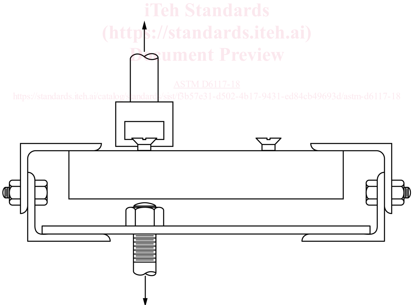
FIG. 1 Diagram of Assembly for Screw Withdrawal Test
