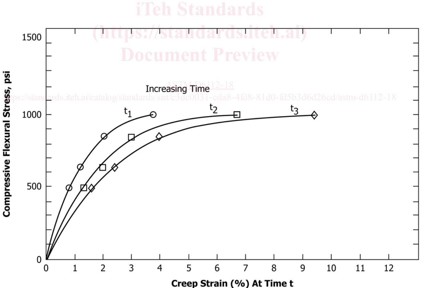
FIG. 2 Cartesian Isochronous Stress Strain Curves at Various Times
