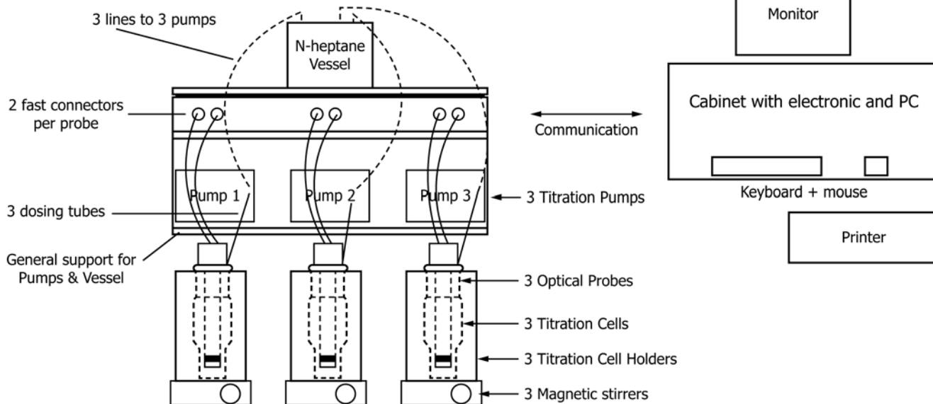
FIG. 1 Schematic Drawing of the Integrated Automated Stability Analyser System
