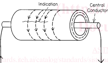
FIG. 4 Circular Magnetization, Current Through a Conductor
