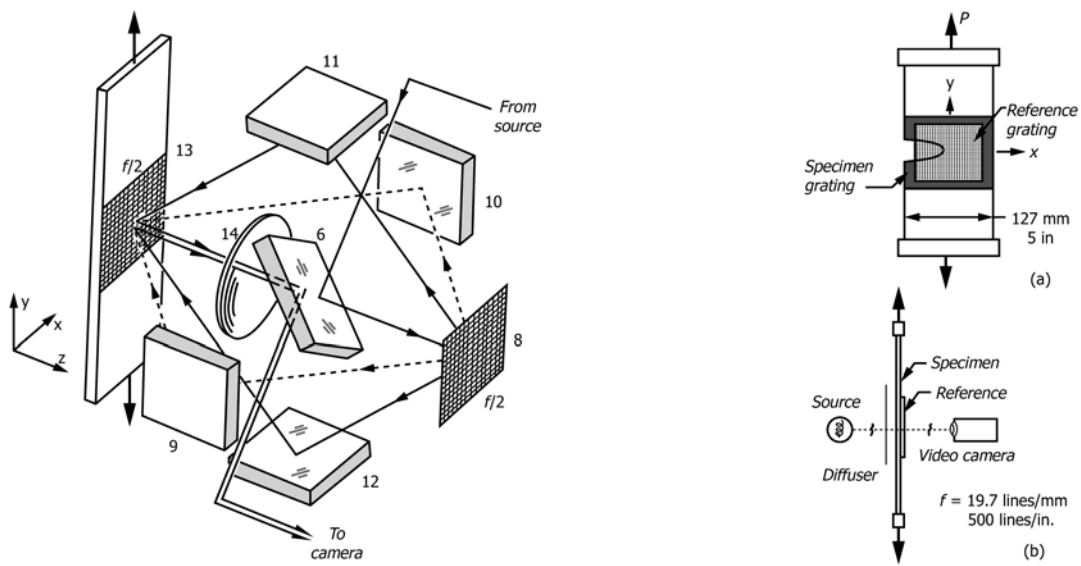
(a) Compact moiré interferometer
