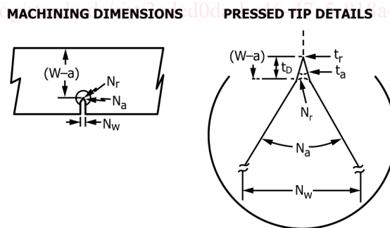
Dimensions and Tolerances for Notch Tip
