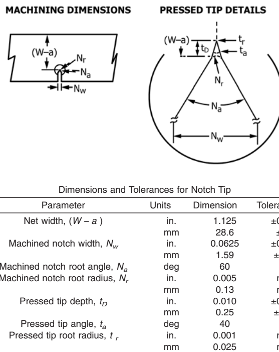
FIG. 2 Details of the Notch in a Dynamic Tear Specimen
