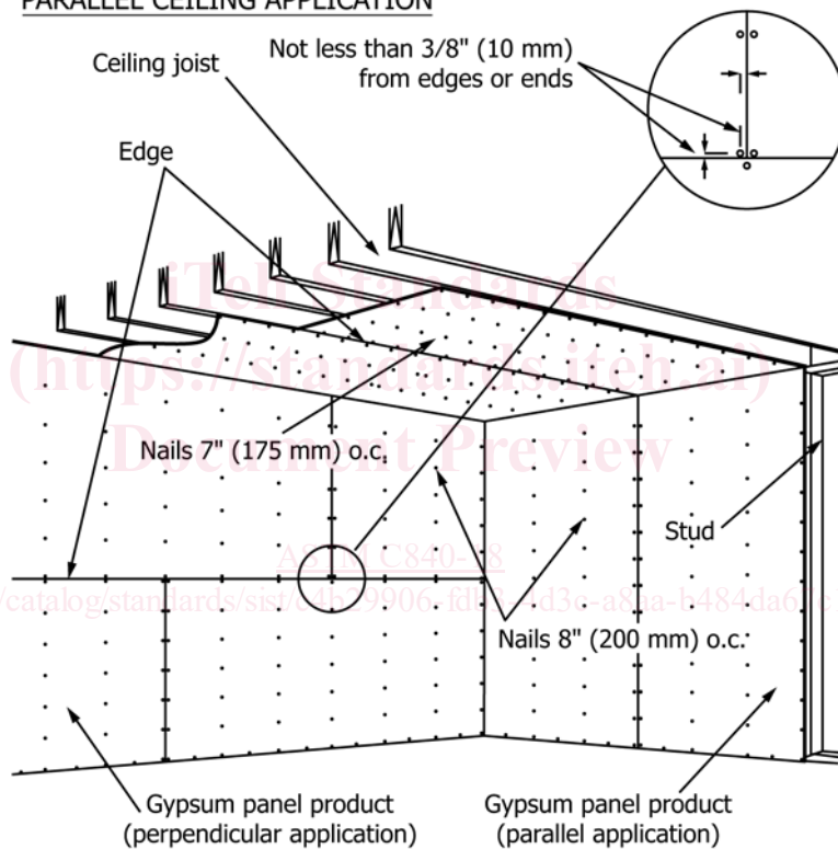
FIG. 2 Single Nailing
