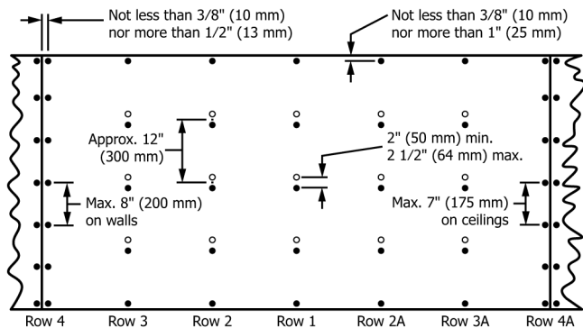
FIG. 3 Double Nailing
