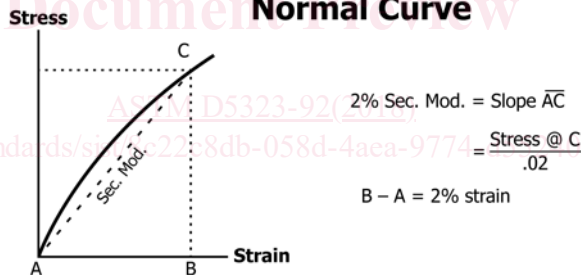
FIG. X1.1 Normal Curve
