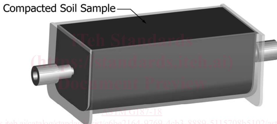
FIG. 2 Typical Two-Electrode Soil Box (Empty and Full)
