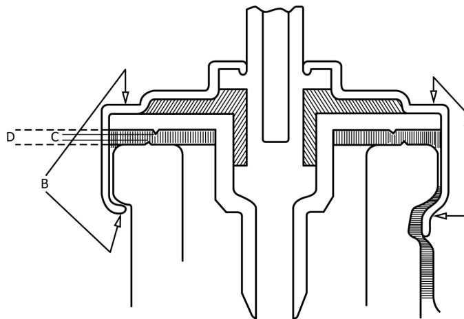
A—points between which effective crimp height measurement should be made (these points are self-determining when the calipers are held parallel to the side of the valve). B—points between which a relative measurement may be established for nondestructure quality control use from optical comparator data. C—effective compression. D—flat compression.
