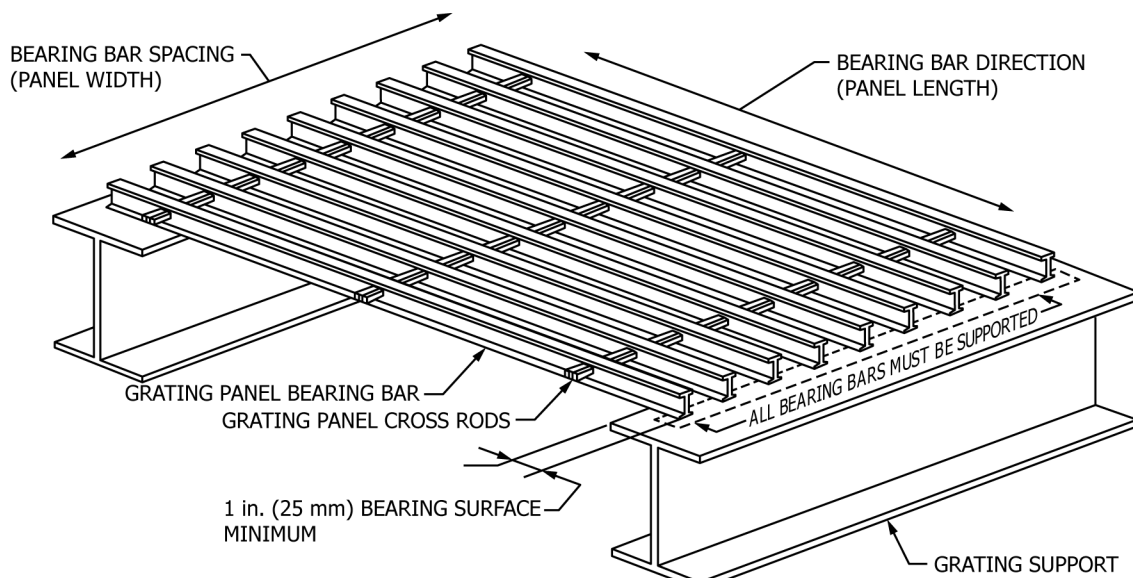
FIG. 3 Pultruded Grating
