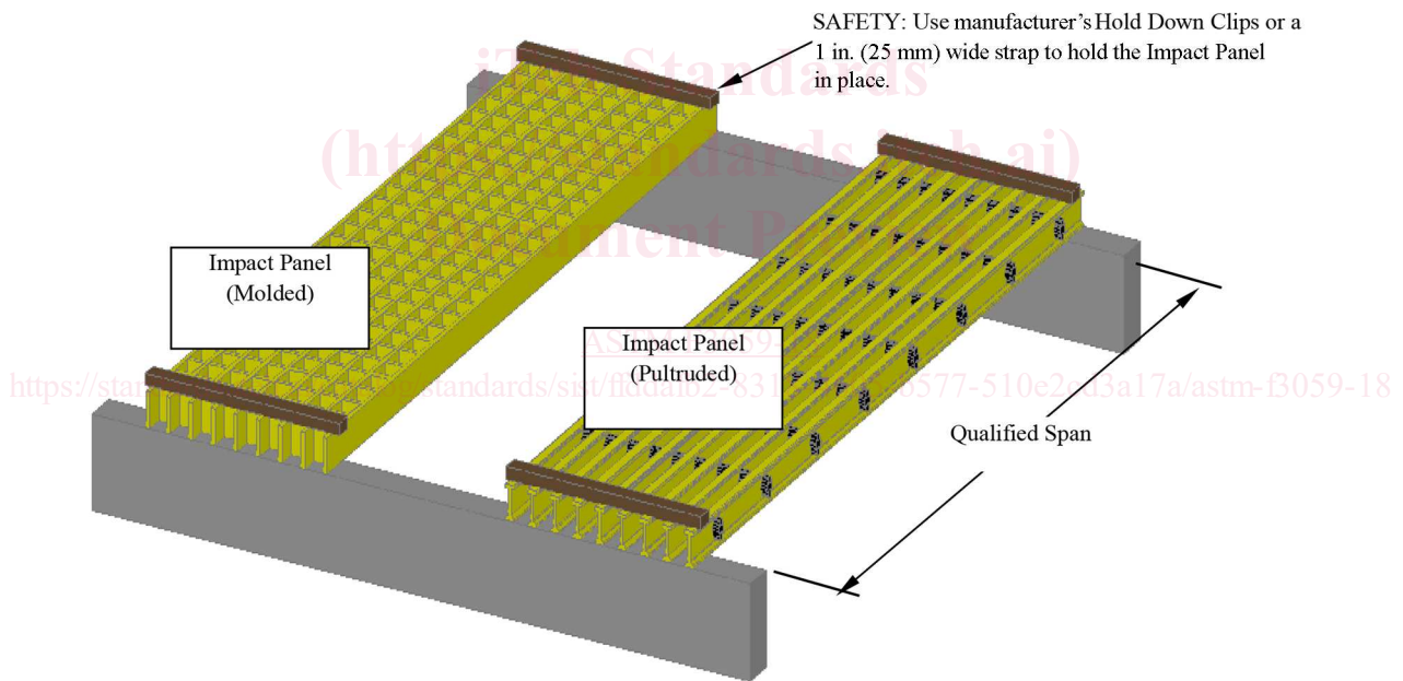
FIG. 5 Impact Panel Simply Supported at the Qualified Span
