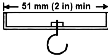
FIG. A1.2 Lid and Hook
