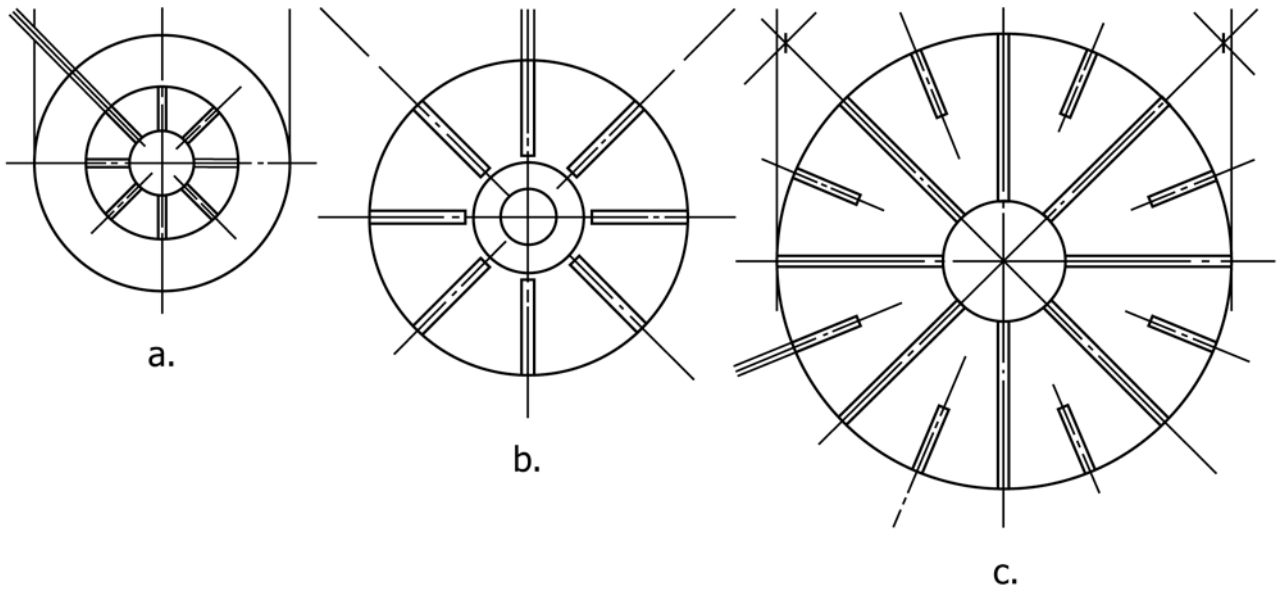
FIG. 3 Vane Configuration (a) High Capacity, (b) Standard, (c) Sensitive
