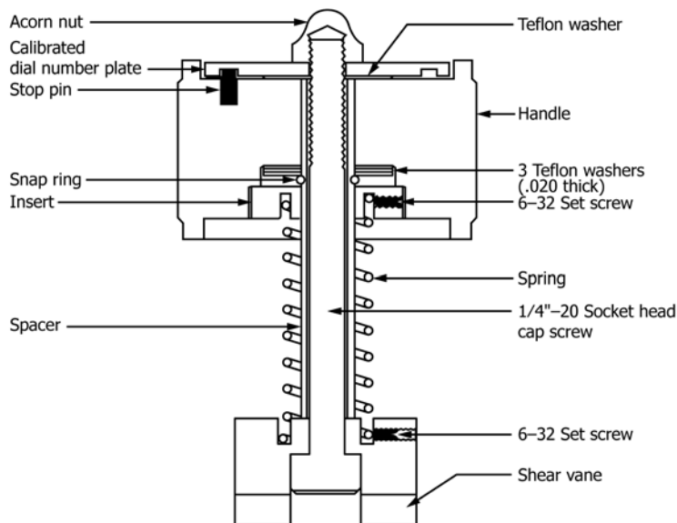
FIG. 2 Example Schematic of the Torsional Shear Device 3,4
