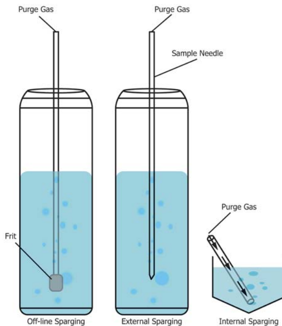
FIG. 1 TIC Removal
