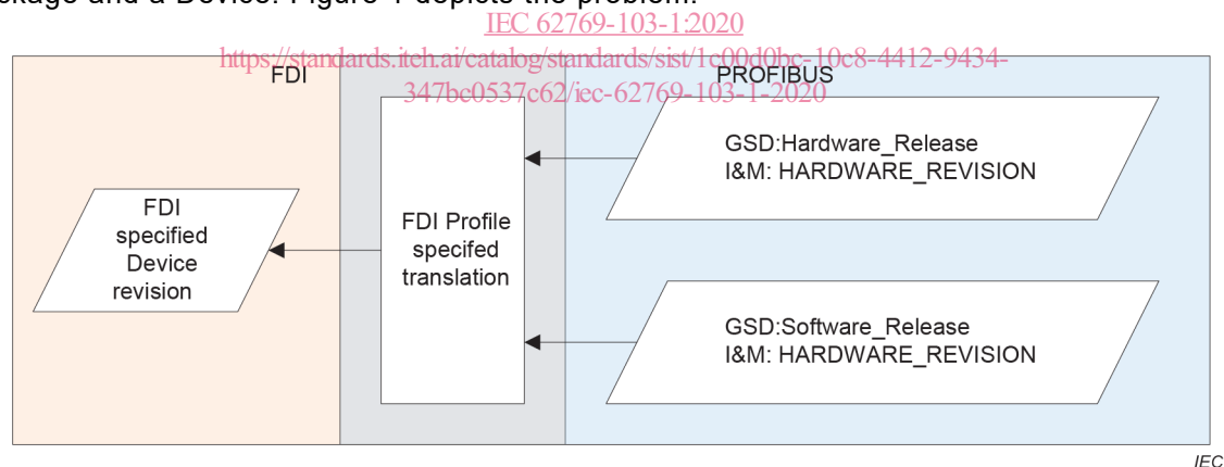
Figure 1 – Version mapping problem
