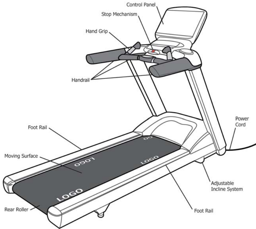
FIG. 1 Treadmill Terminology
