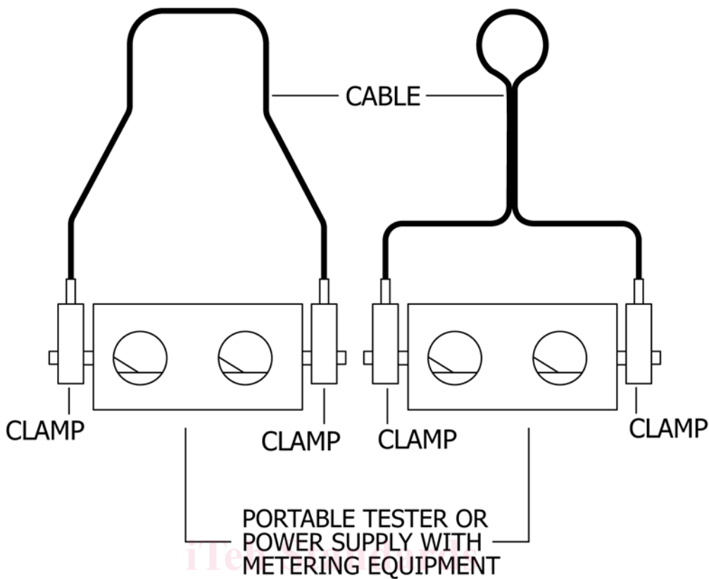
FIG. 2 Typical Configurations
