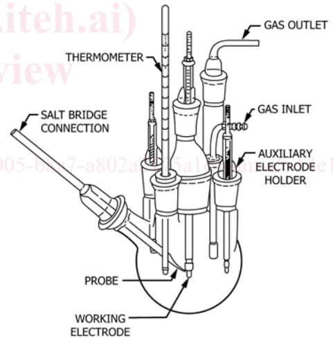
FIG. 2 Schematic Diagram of Polarization Cell (1)
