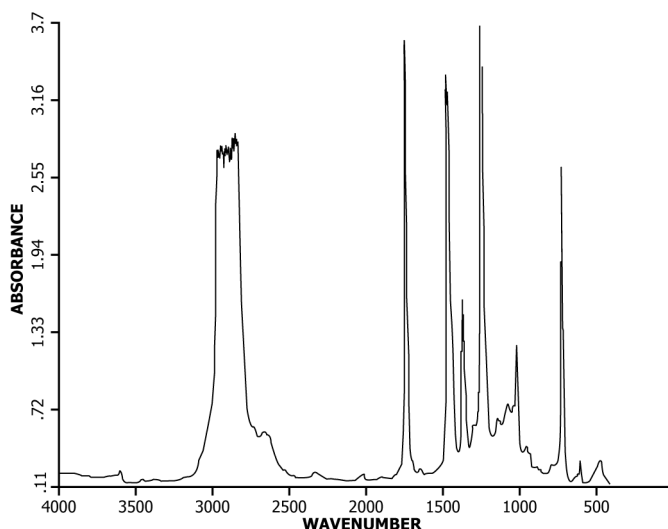
FIG. 1 —FT-IR/FT-IR Spectrum of EVA Copolymer Standard (4.8 % Vinyl Acetate) Analyzed by Procedure B
