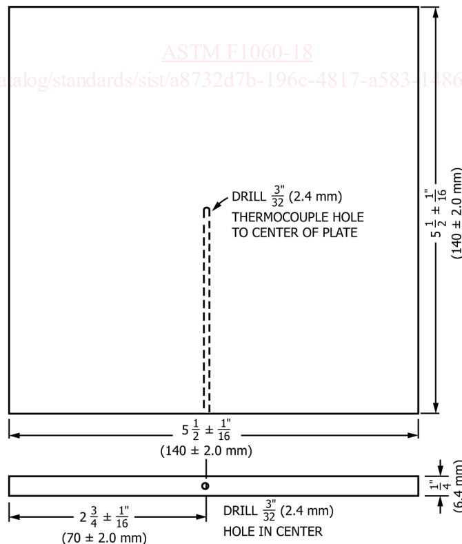
FIG. 2 Surface Plate
