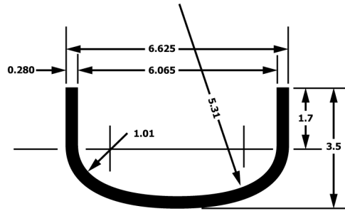
FIG. 4 Nominal 6 in. Weld Cap Weight (Approximately) 6.4 lb
