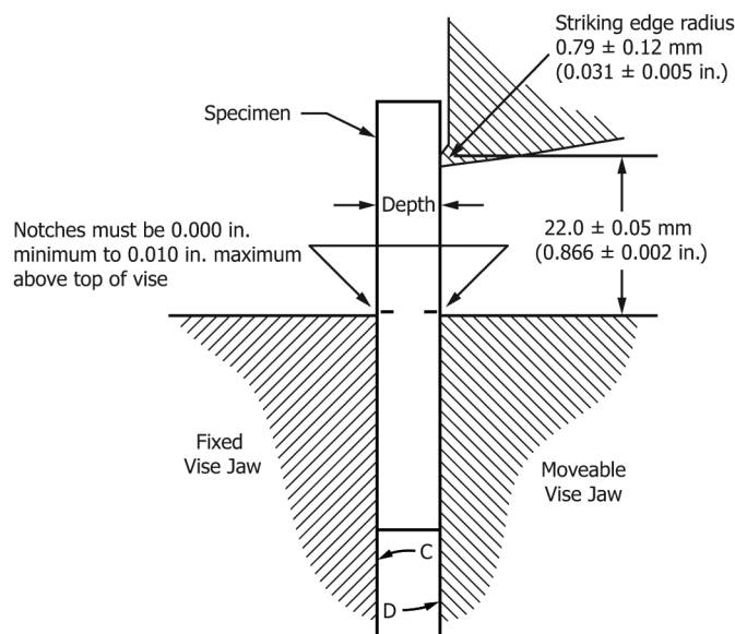
FIG. X2-2A3.2 Relationship of Vise, Specimen, and Strike Edge to One Another
