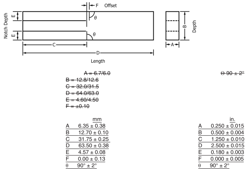
FIG. X2-1A3.1 Dimensions of Double-Notched Izod Test Specimens
