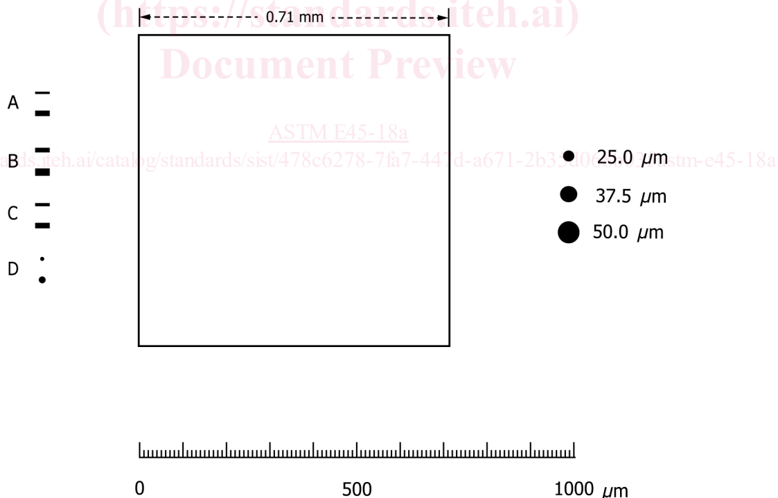
FIG. 5 Suggested Reticle or Overlay Grid For Methods A, D, and E
