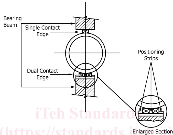
FIG. 2 Loading Apparatus
