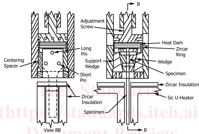
FIG. 6 Example of Pin/Face-Loaded Pin/Face-Loaded, Passive Grip Interface (5)
