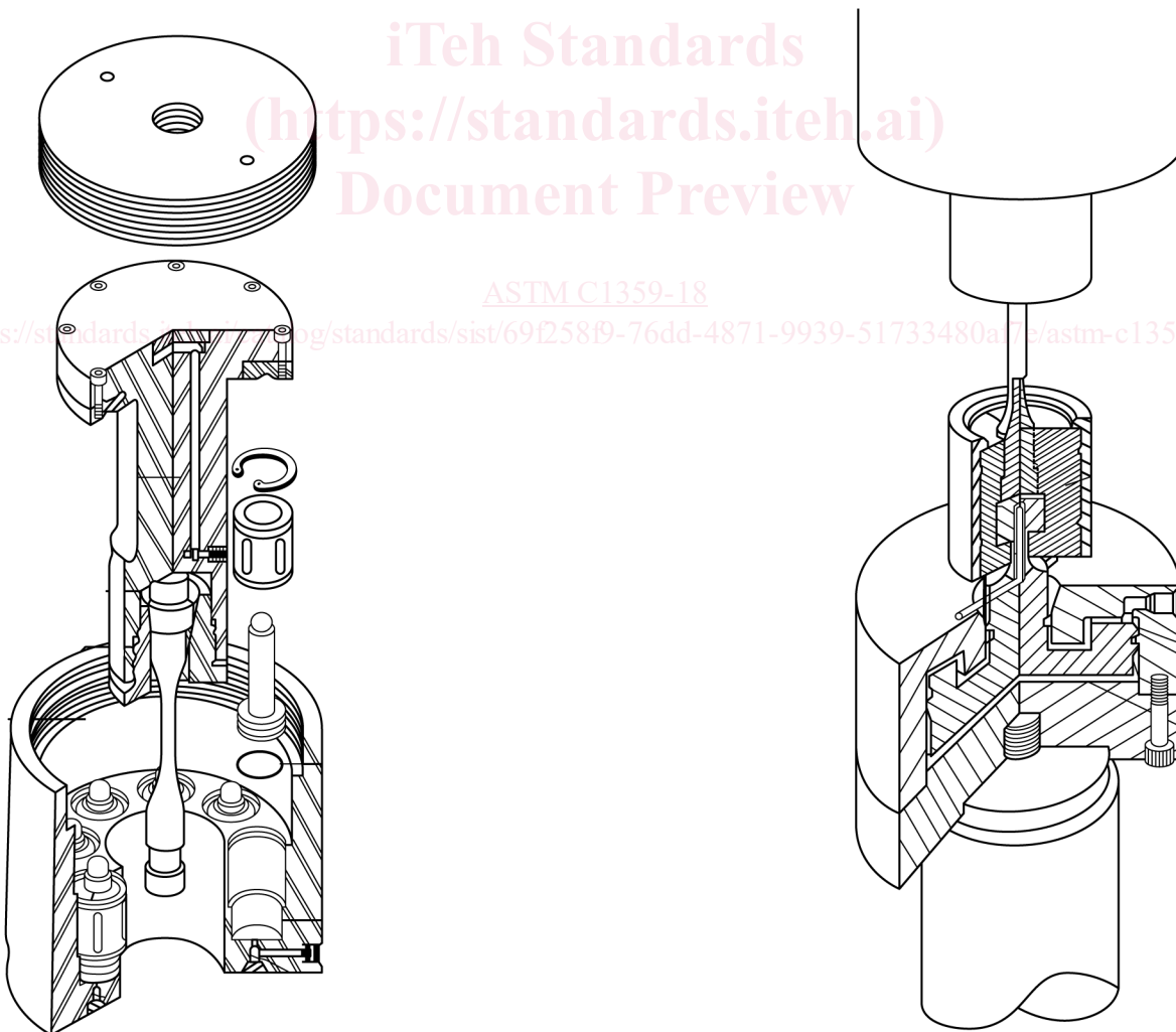
FIG. 7 Examples of Hydraulic, Self-Aligning, Non-Fixed-Non-Fixed Load Train Couplers (9, 10)
