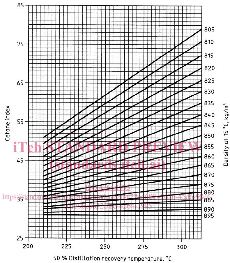
Figure 1 — Cetane index — Estimate based on density and 50 % distillation recovery temperature
