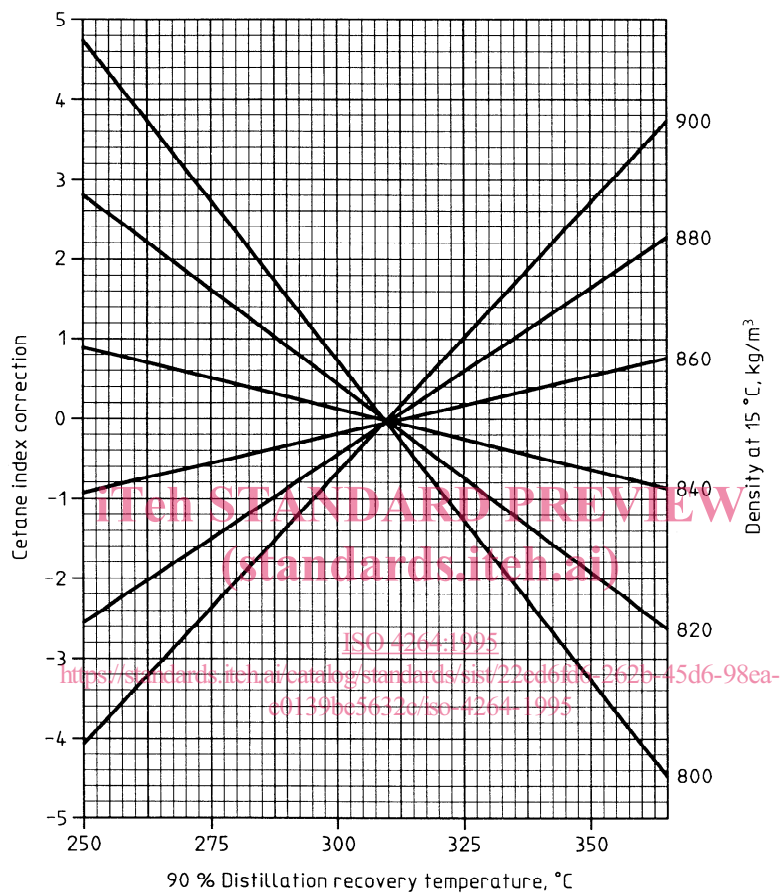
Figure 2 — Cetane index — Correction for deviations from average values in density and 90 % distillation recovery temperature
