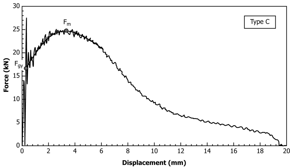
FIG. 2 Characteristic Force-Displacement Curves and Definitions of Characteristic Forces
