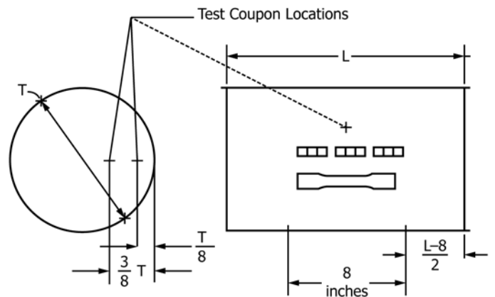
FIG. 1 Test Block Configuration
