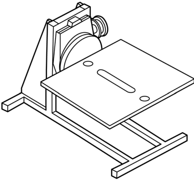
FIG. 4 Example of Specimen Holder Using Machinist's Rotary Table
