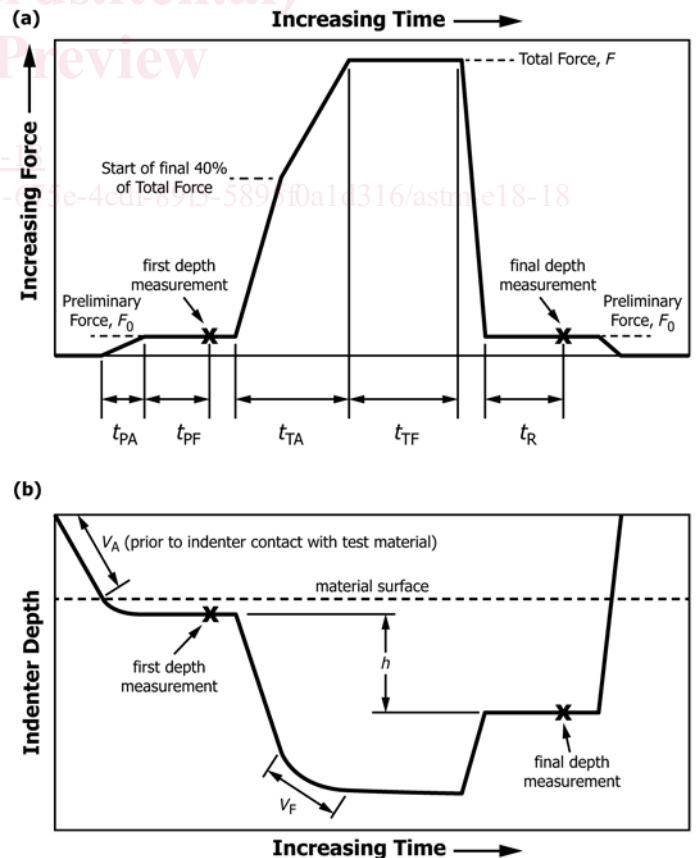
FIG. 2 Schematic of Force-Time Plot (a) and Indenter Depth-Time Plot (b) of an HRC Test Illustrating the Test Cycle Parts
