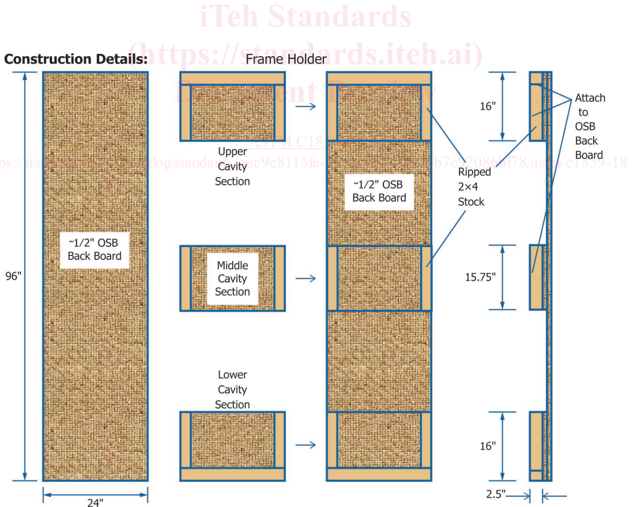
FIG. 1 Recommended Frame Holder (an Example)
