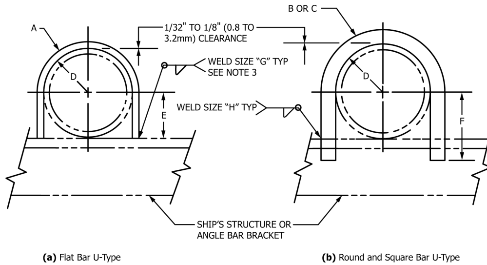
FIG. 2 Strap Hangers
