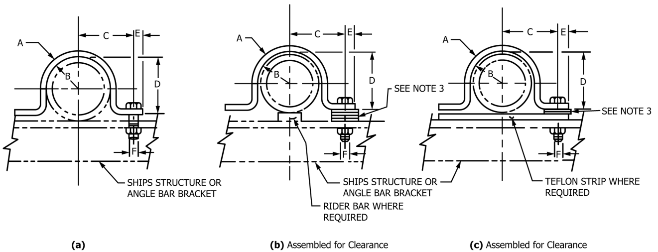
FIG. 1 Split Cap Hangers
