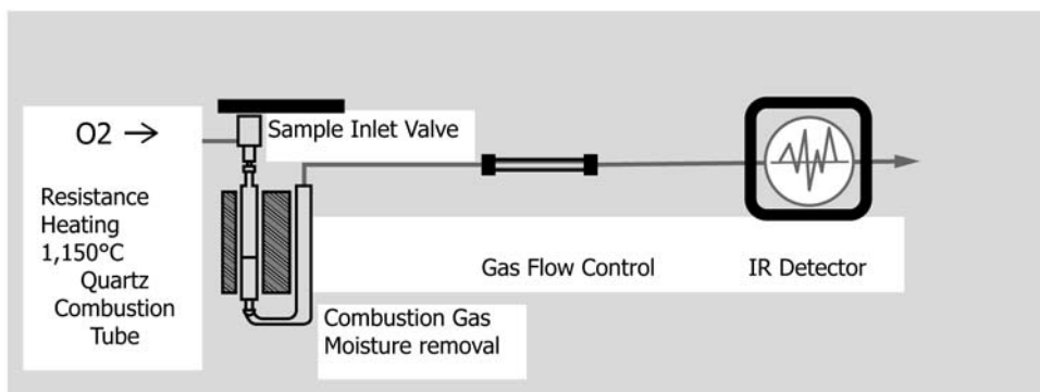
FIG. 2 Apparatus for Determination of Sulfur by Infrared Detection, Method B
