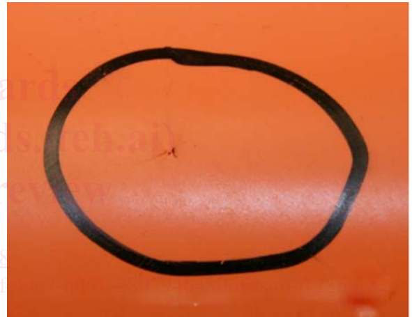
FIG. 5 Breakdown (Dielectric Failure Blanket: Front)
