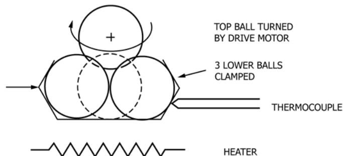
FIG. 1 Schematic of a Four-Ball Wear Test Machine
