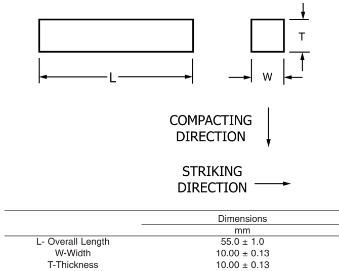
FIG. 3 Unnotched Charpy (Simple Beam) Impact Test Specimen for Metal Powder Structural Materials
