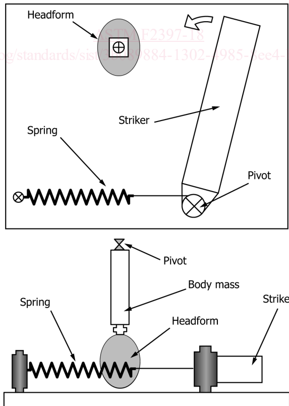
FIG. 1 Striking Impact Test.
