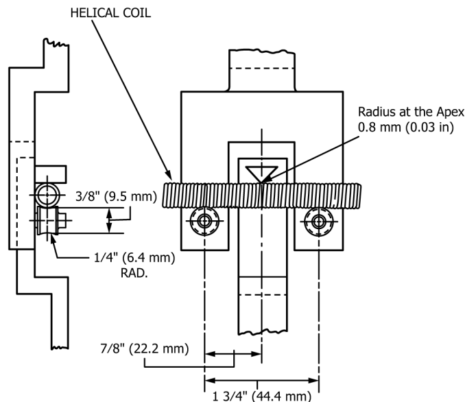
FIG. 1 Test Fixture for Bond Strength Test
