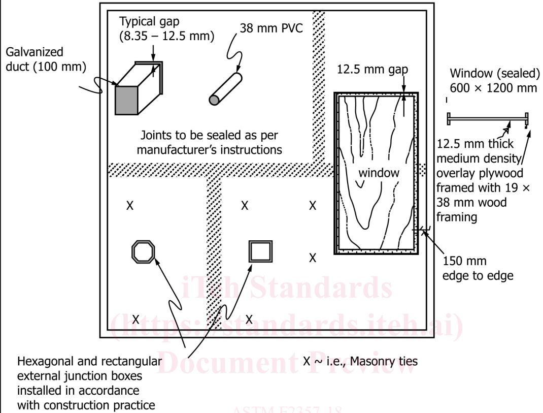
FIG. A1.2 Specimen 2—Continuity at Penetrations- fbbf3747bd29/astm-e2357-18
