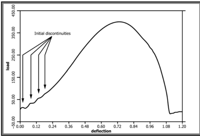
FIG. X1.1 Inertial Effect
