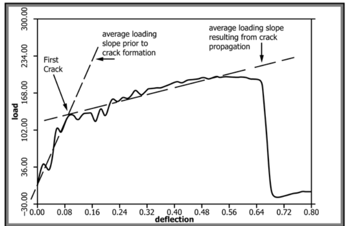
FIG. X1.3 First Crack Determination
